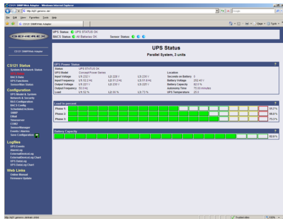
UPSMAN on CS121/CS141 – Web-Browser Configuration/Monitoring
